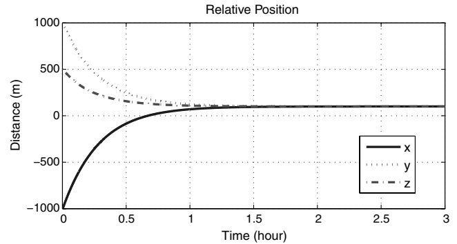
Fig. 3 Relative position regulation in an elliptical orbit by control law (16).
